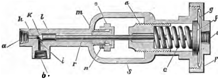
FIG. 206.—The "Locke" Diaphragm Fuel Feed Regulator. Unlike the one shown in Fig. 207, this device is constructed to operate with some firing device other than a "torch." The parts shown are: a , gasoline supply pipe, whose opening is regulated by point, k , on valve head, l ; b , gasoline delivery to burner; c , steam inlet; g , diaphragm; f , pressure head; r , valve rod; o , packing nut; n , gland; m , asbestos spring packing; a , main frame; d , adjusting screw for regulating tension of spring; e ; p , cover of pressure chamber, screwed to head of m , as indicated.
